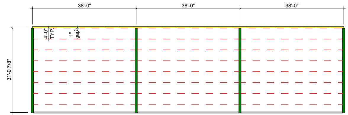
12P DEEP GRID (adding 4' hollow core)
