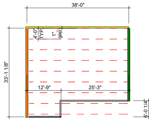
4P CORNER GRID
