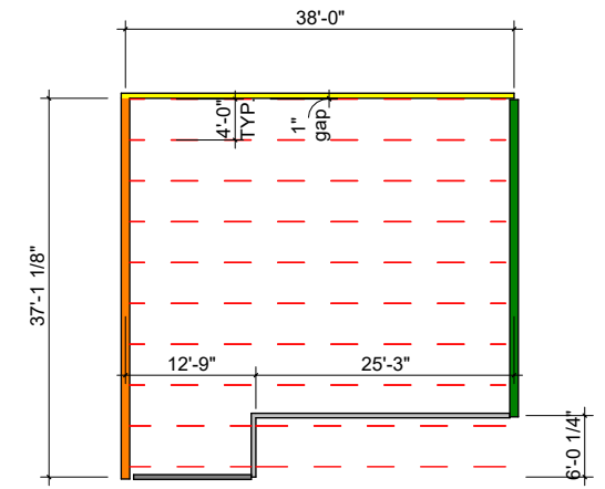
4P DEEP CORNER GRID (adding 4' hollow core)
